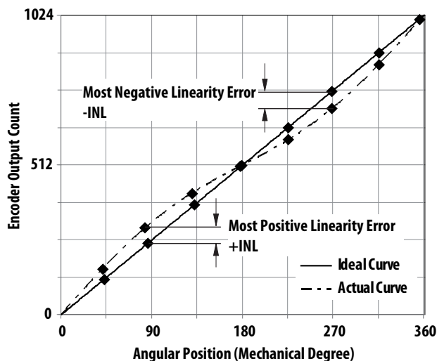
Figure 3. Integral non-linearity
